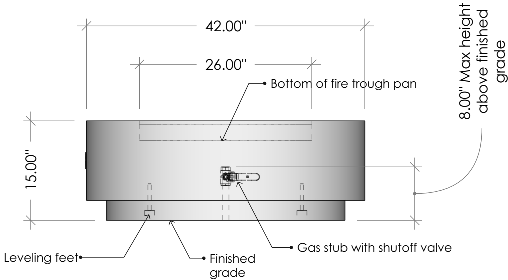
FRONT VIEW
