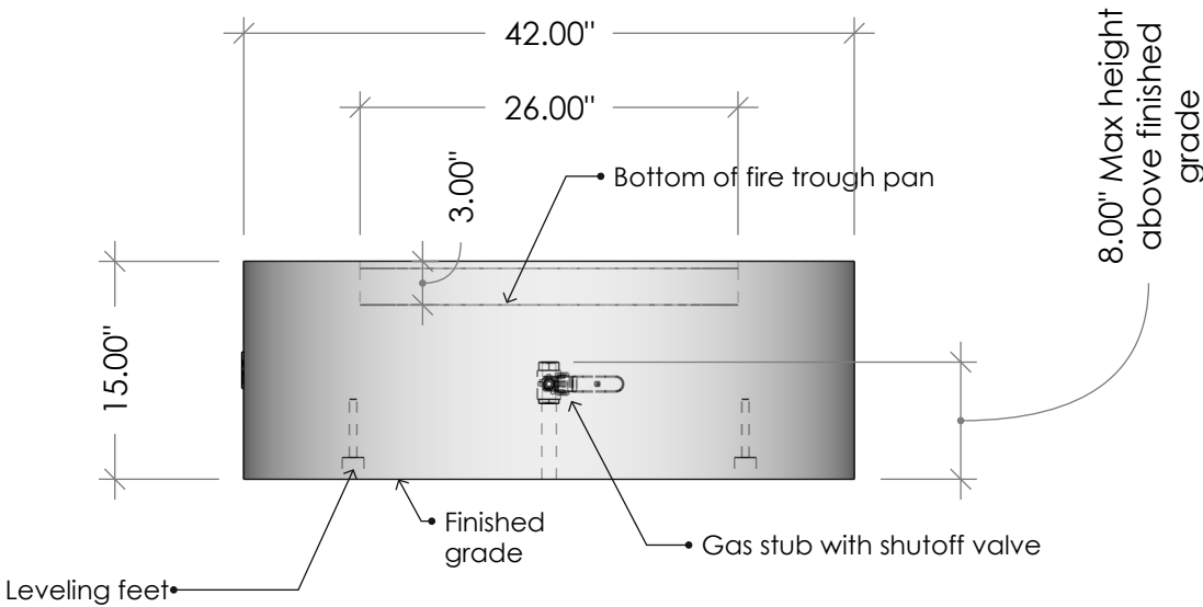
FRONT VIEW
