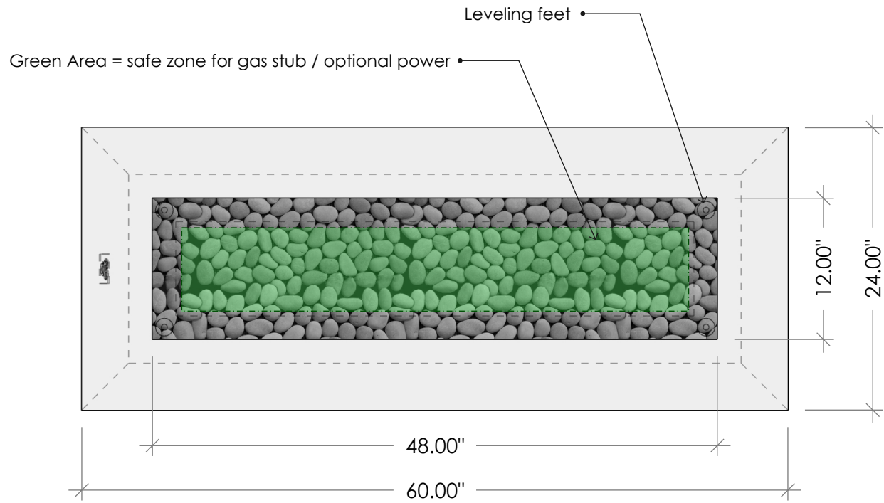
TOP VIEW
