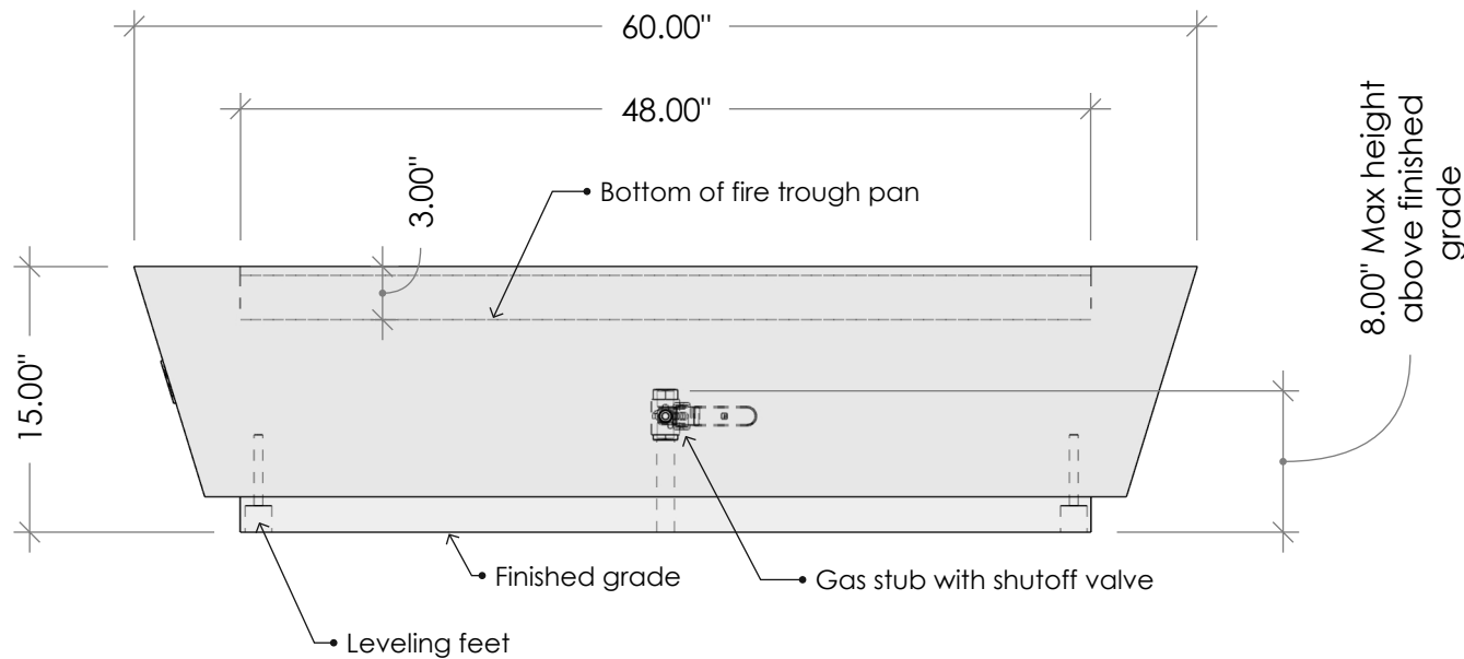
FRONT VIEW
