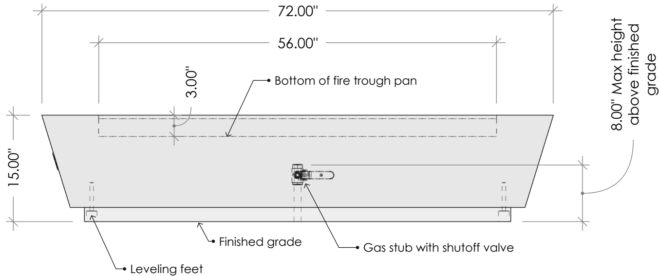
FRONT VIEW
