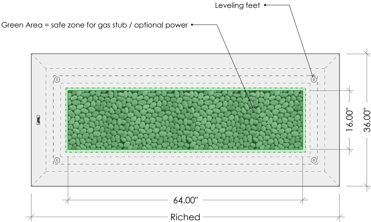
TOP VIEW
