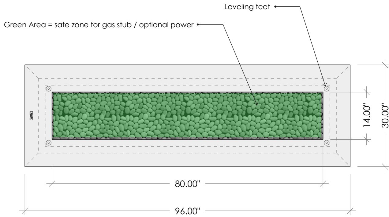
TOP VIEW
