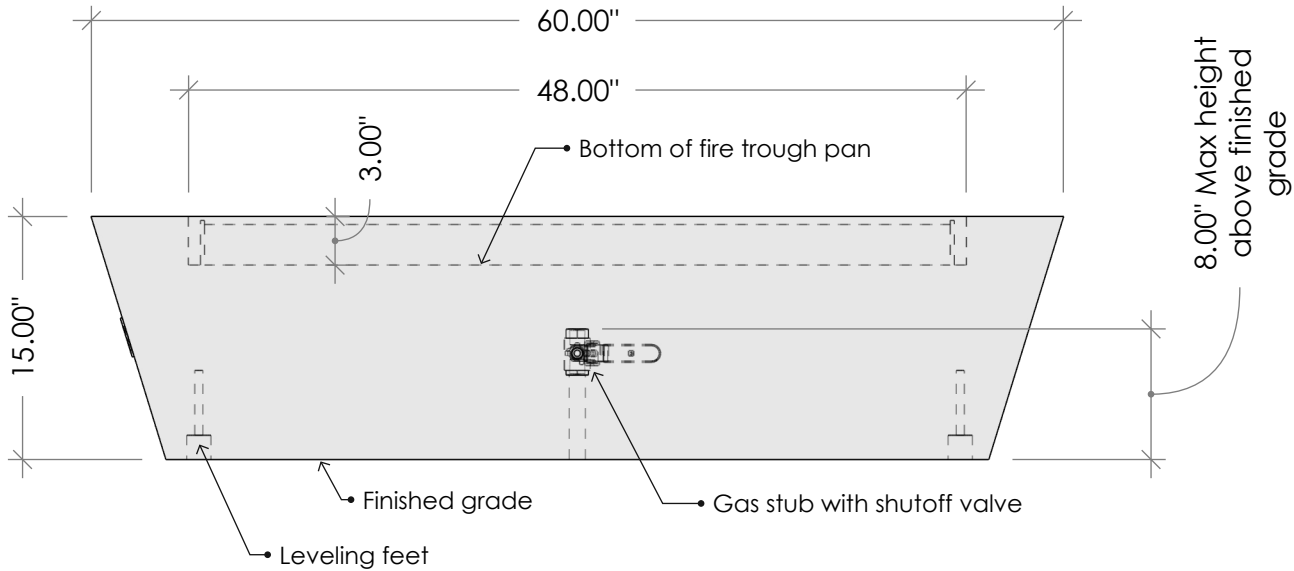
FRONT VIEW
