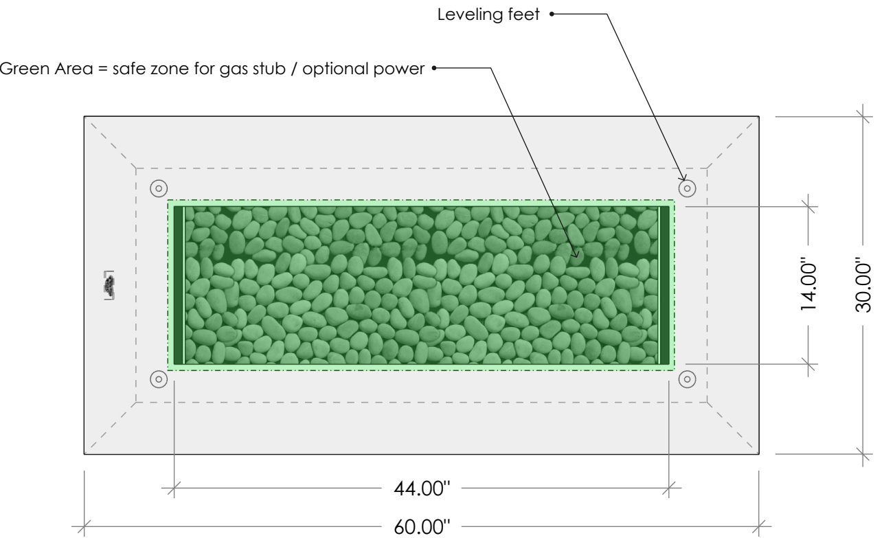
TOP VIEW
