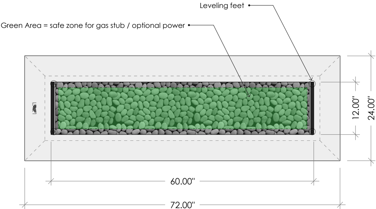
TOP VIEW
