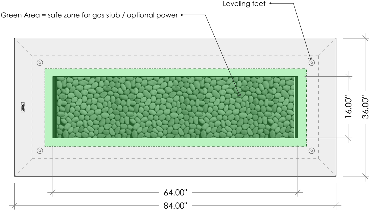
TOP VIEW
