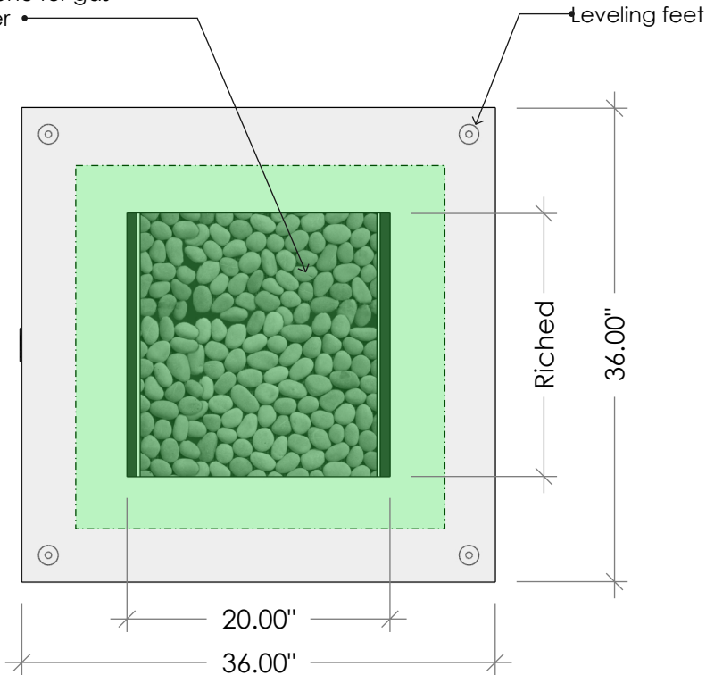
TOP VIEW
