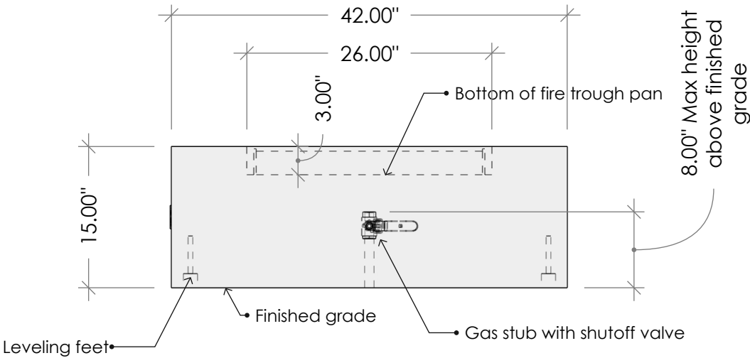
FRONT VIEW
