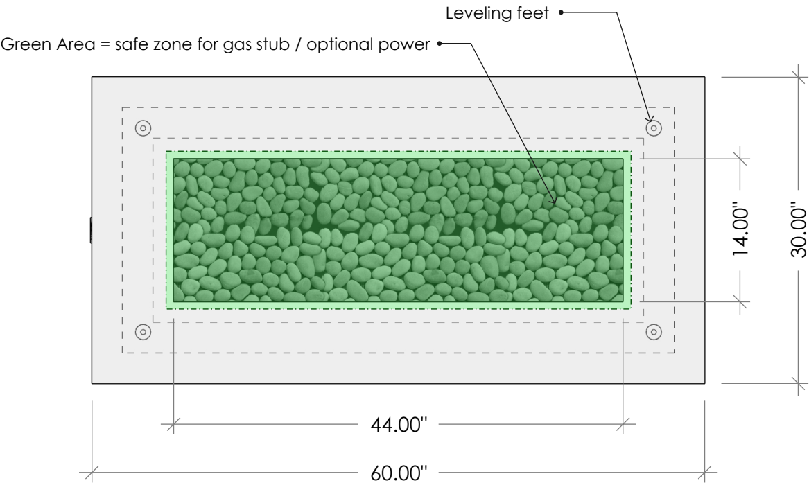
TOP VIEW
