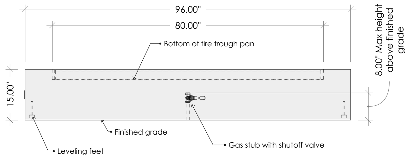
FRONT VIEW
